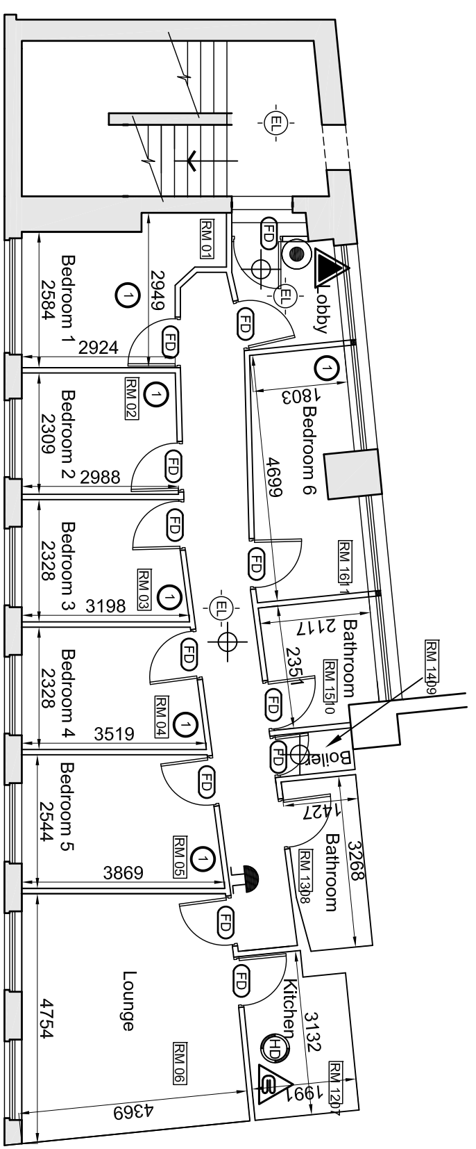
Existing Third Floor Plan
